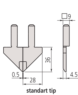
standart tip
